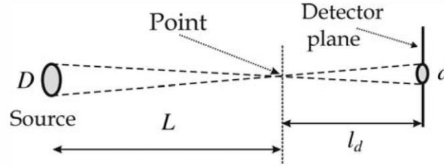
Figure 6. The role of the collimation ratio in the blurring effects
