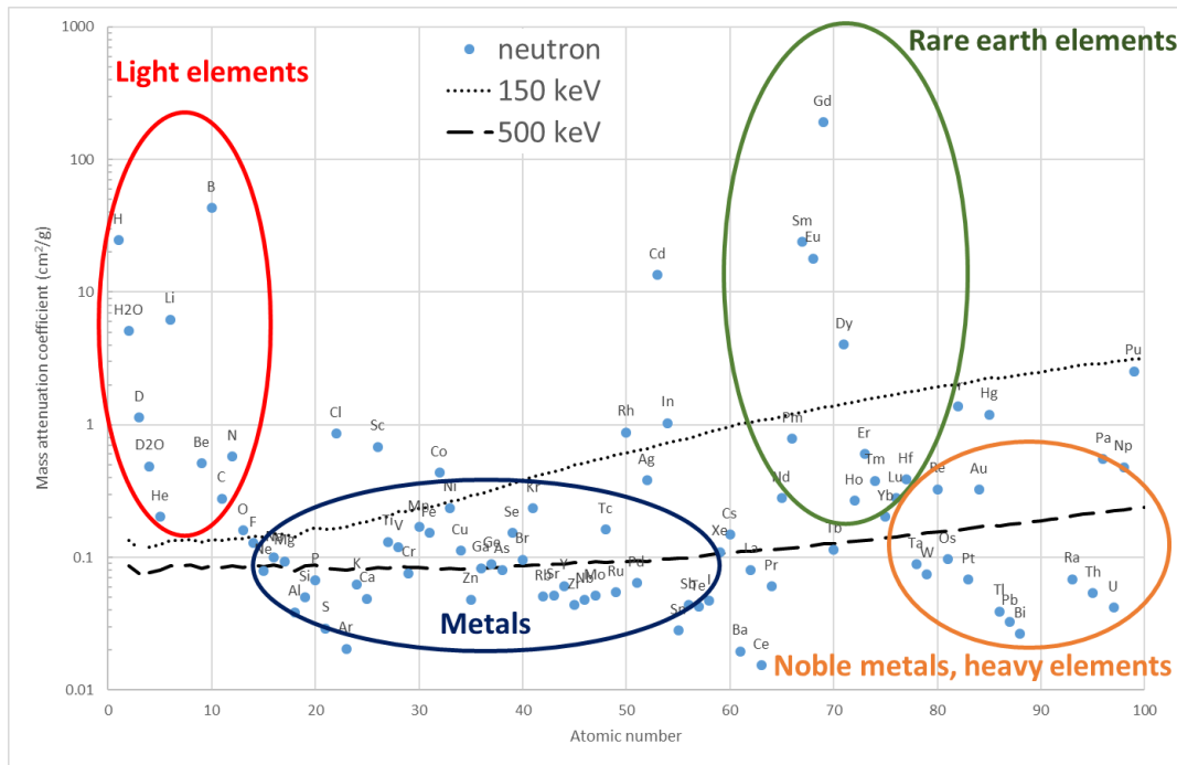
Figure 2. Mass attenuation coefficients of elements on logarithmic scale for thermal neutrons (dots), for 500 keV gamma radiation (dashed line), for 150 kV X-ray (dotted line)
