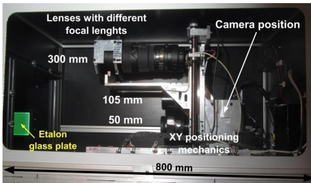
Figure 9. The light-tight box and the opto-mechanical system of the RAD facility
