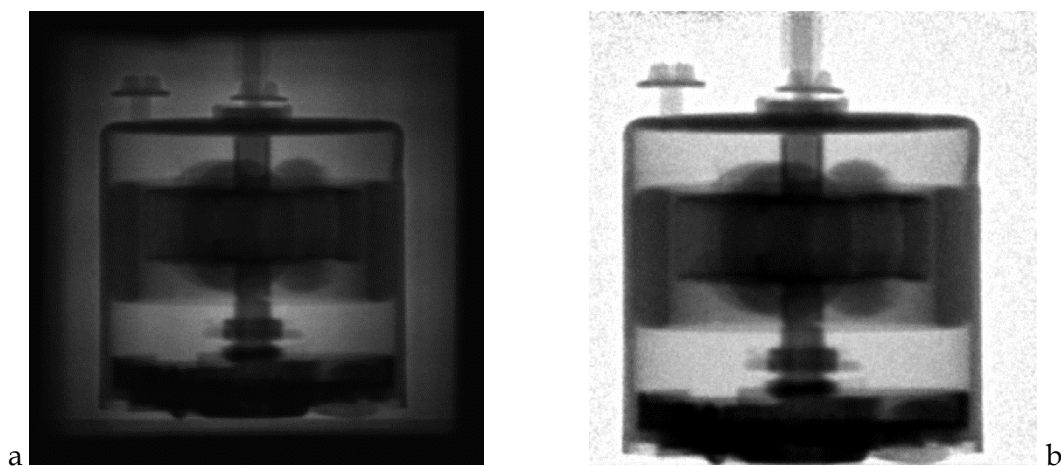
Figure 5. The raw (a) and the normalized (b) neutron radiographic image of a stepper motor
