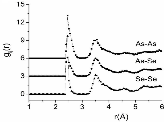
Figure 9. The partial pair correlation functions, obtained from RMC modelling of \text{As}_2\text{Se}_3 composition
