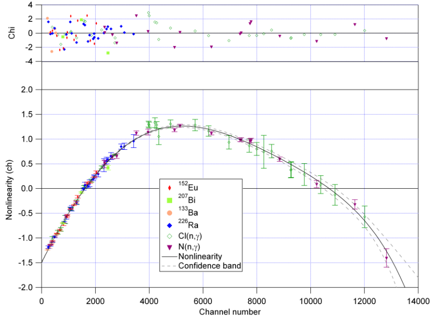
Figure 5. Nonlinearity of the Budapest PGAA system
