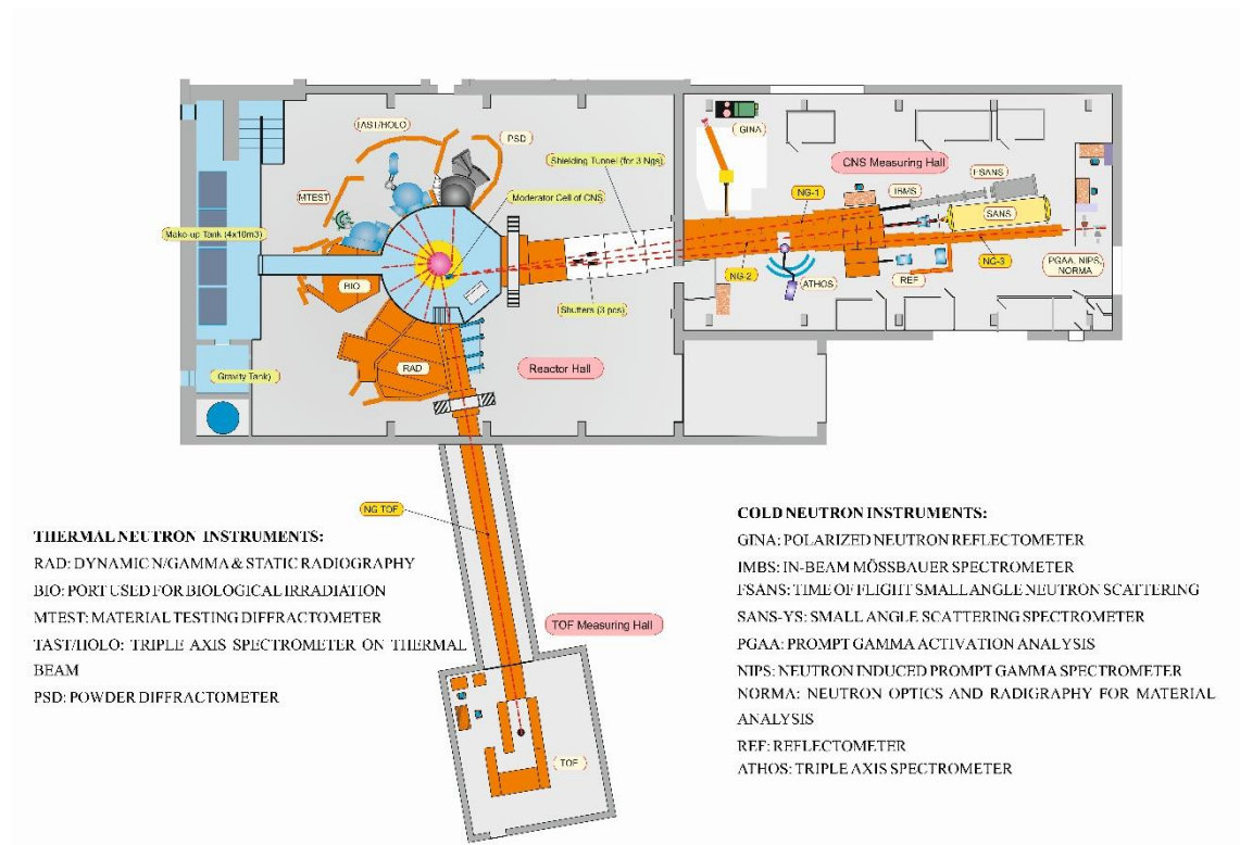
Figure 10. Layout of the horizontal neutron beam facilities at the Budapest Research Reactor
