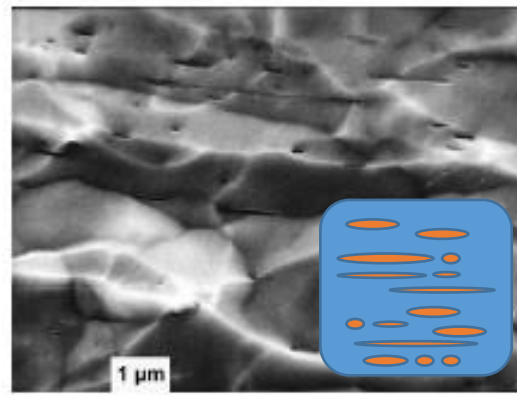
Figure 1. SEM picture and constructed model of potassium bubbles (orange) in tungsten matrix (blue) (SEM picture from: L. Bartha, P. Harmat, O. Horacsek, T. Grósz, L. Rosta: Proceedings on 4 th International Conference on Tungsten (1998) 203-210)
