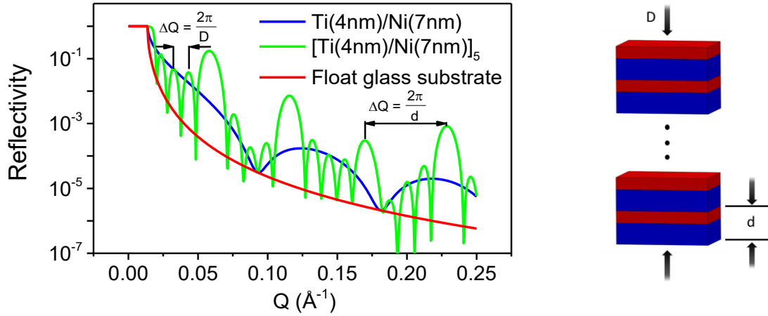
Figure 3. Neutron reflectivity of the [\text{Ti}(4\text{nm})/\text{Ni}(7\text{nm})]_5 multilayer (green) and of the respective Ti/Ni bilayer (blue) along with that of the float glass substrate (red). The bilayer thickness and the total thickness – demonstrated on the right – are in reciprocal relation to the Bragg peak distance and the Kiessig oscillation period, respectively.
