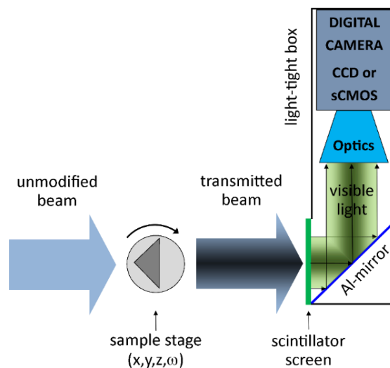
Figure 4. Sketch of a modern radiograph/tomograph setup.
